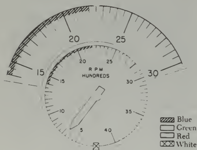
FIGURE 10-28. Tachometer.
